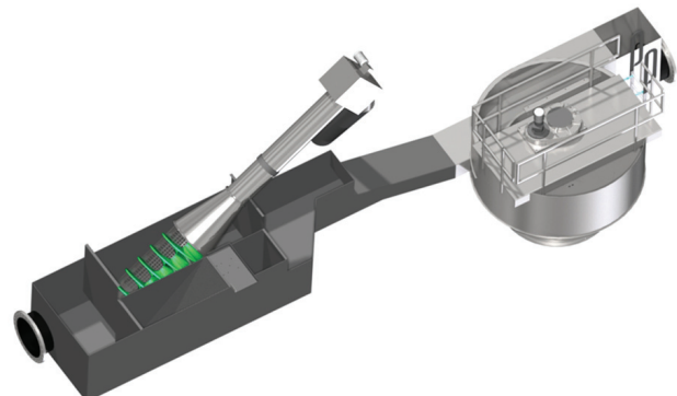
3D model of the inlet channel mounted OBEX™ Spiral Fine Screen assembly used with PISTA® Works™.
